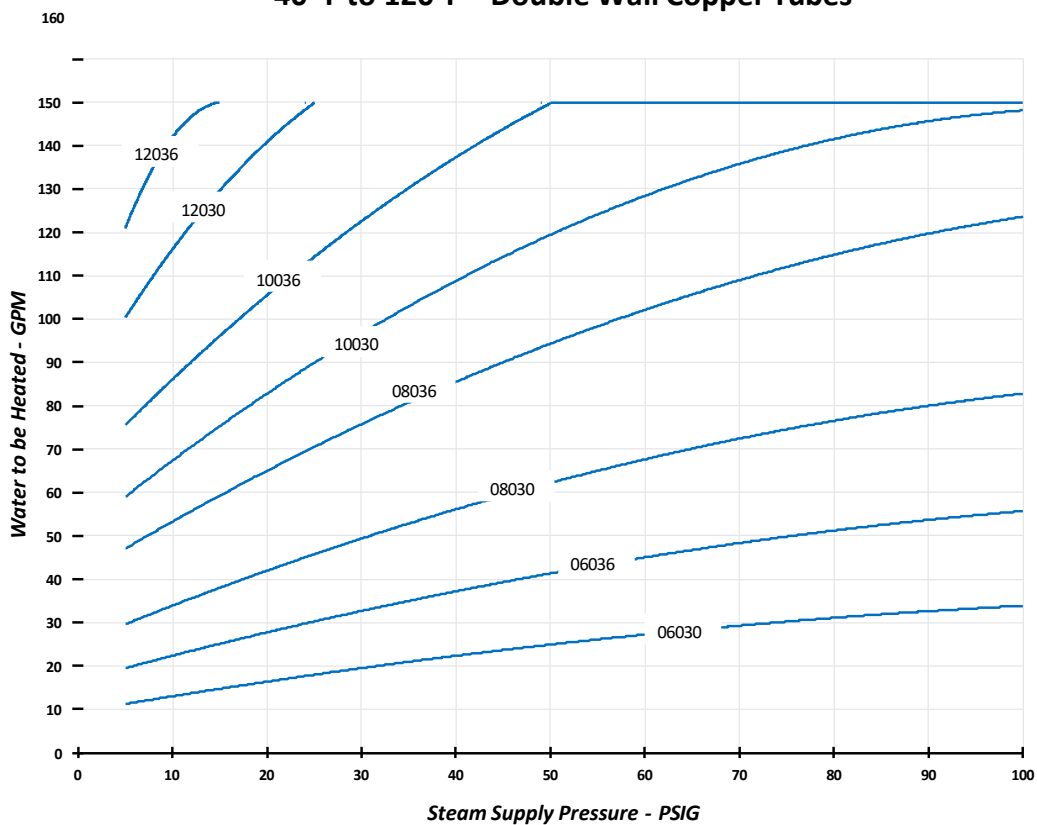
40 °F to 120°F - Double Wall Copper Tubes
