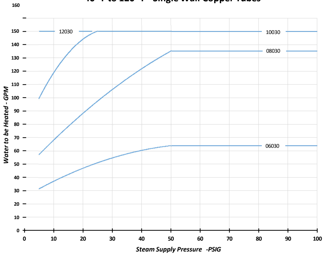
40 °F to 120 °F - Single Wall Copper Tubes
